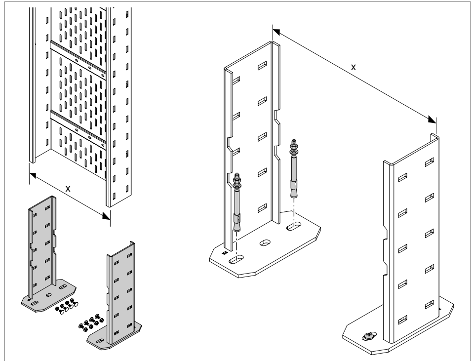
Fig. 28: WFP base plate
