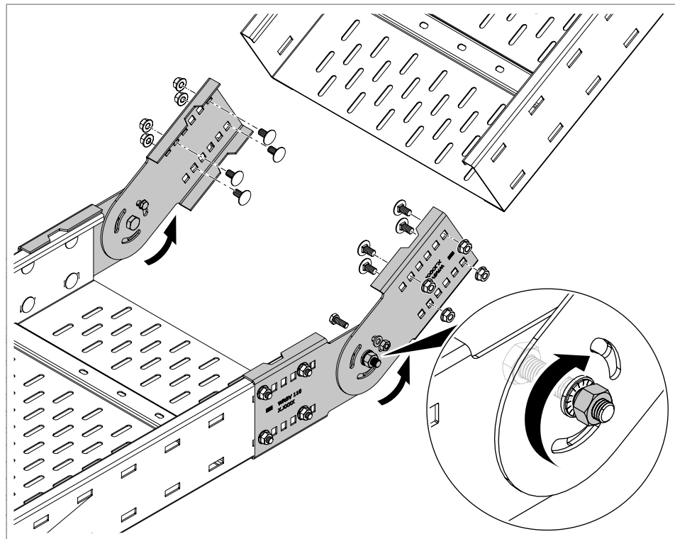
Fig. 23: Adjusting the angle
