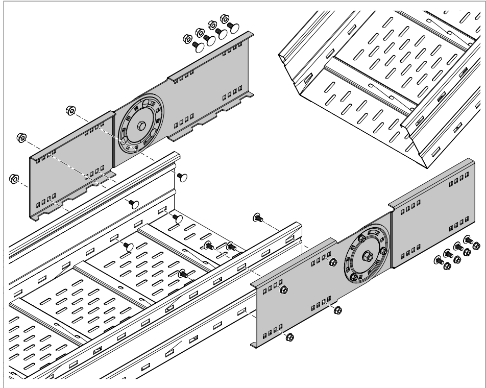
Fig. 25: Applying the adjustable connector
