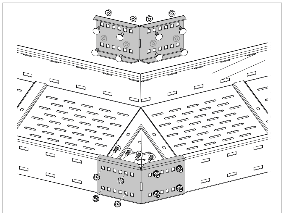
Fig. 18: Screwing on the WRWV angle connector to the inner and outer angle
