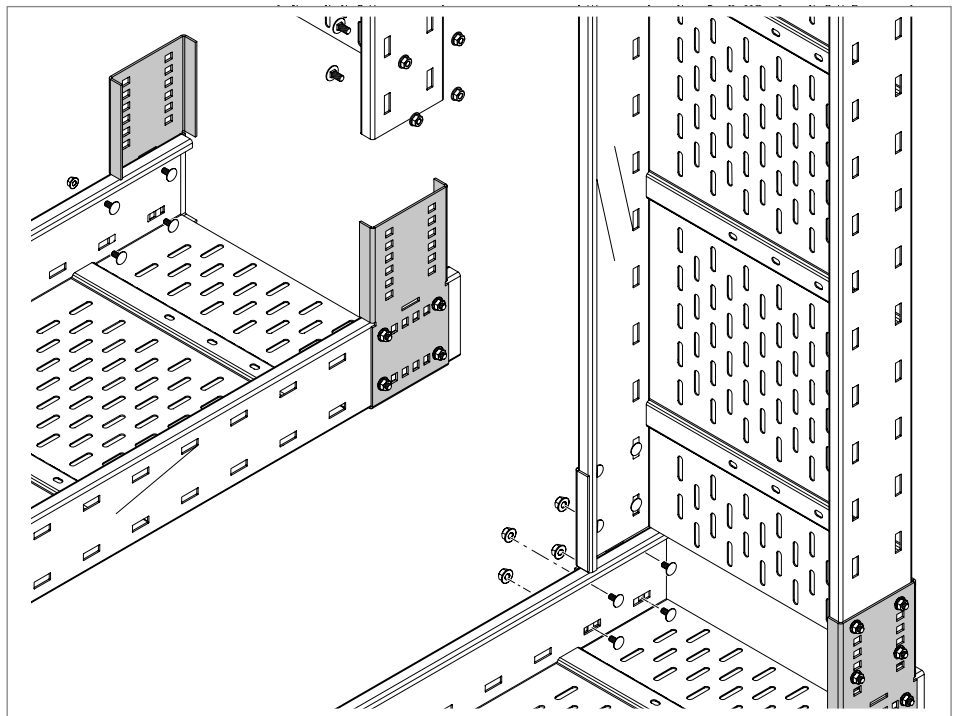
Fig. 20: Screwing on the WRWVV angle connector
