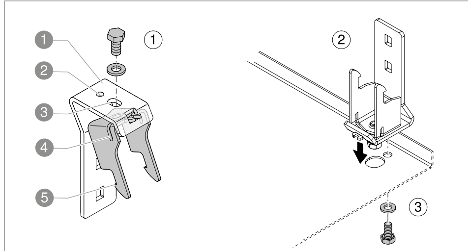
Fig. 47: Mounting spacers on covers
