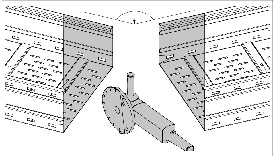
Fig. 14: Cutting the trays to create angles
