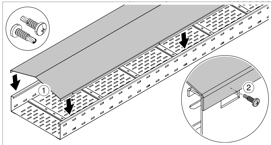
Fig. 43: Place the WDRLU DF cover on the wide span cable tray
