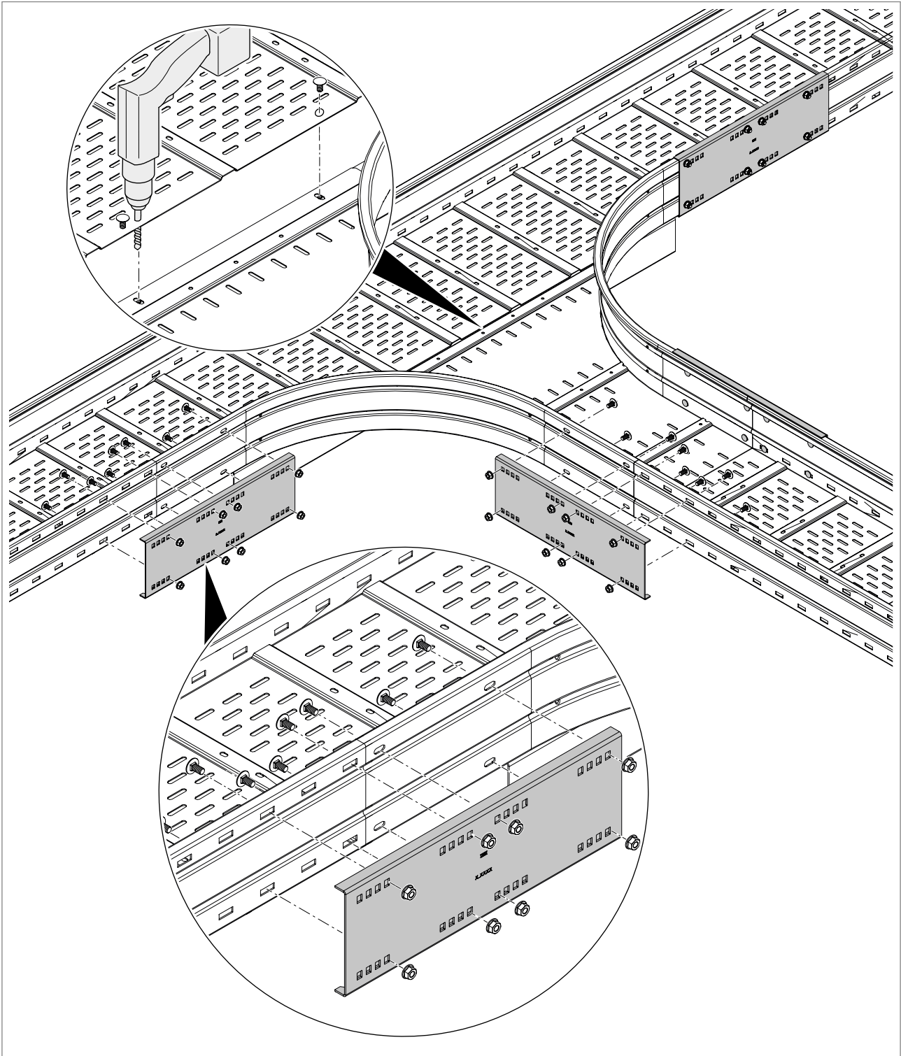
Fig. 37: Screwing on the straight connector
