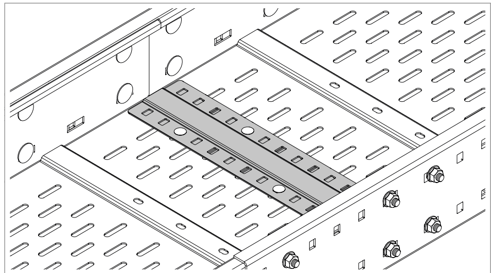
Fig. 13: Mounted joint plate
