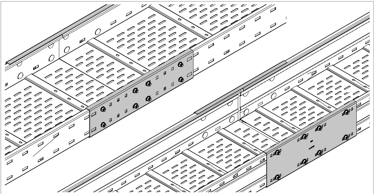
Fig. 11: Screw on the WRVL straight connector
