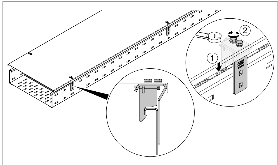
Fig. 49: Mounting the cover on the tray
