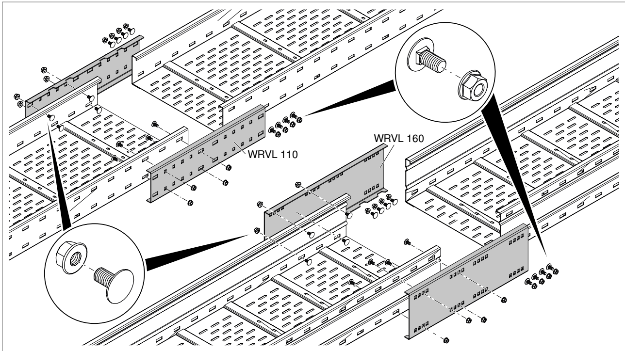
Fig. 10: Applying the WRVL 110 and 160 straight connectors
