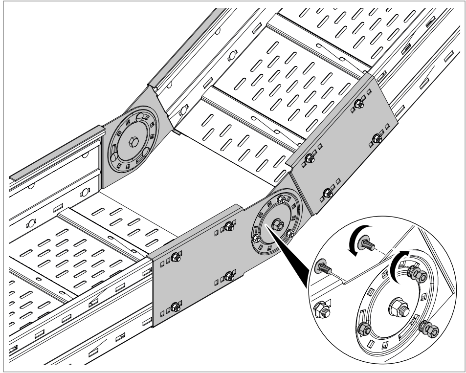
Fig. 27: Mounting the rising tray
