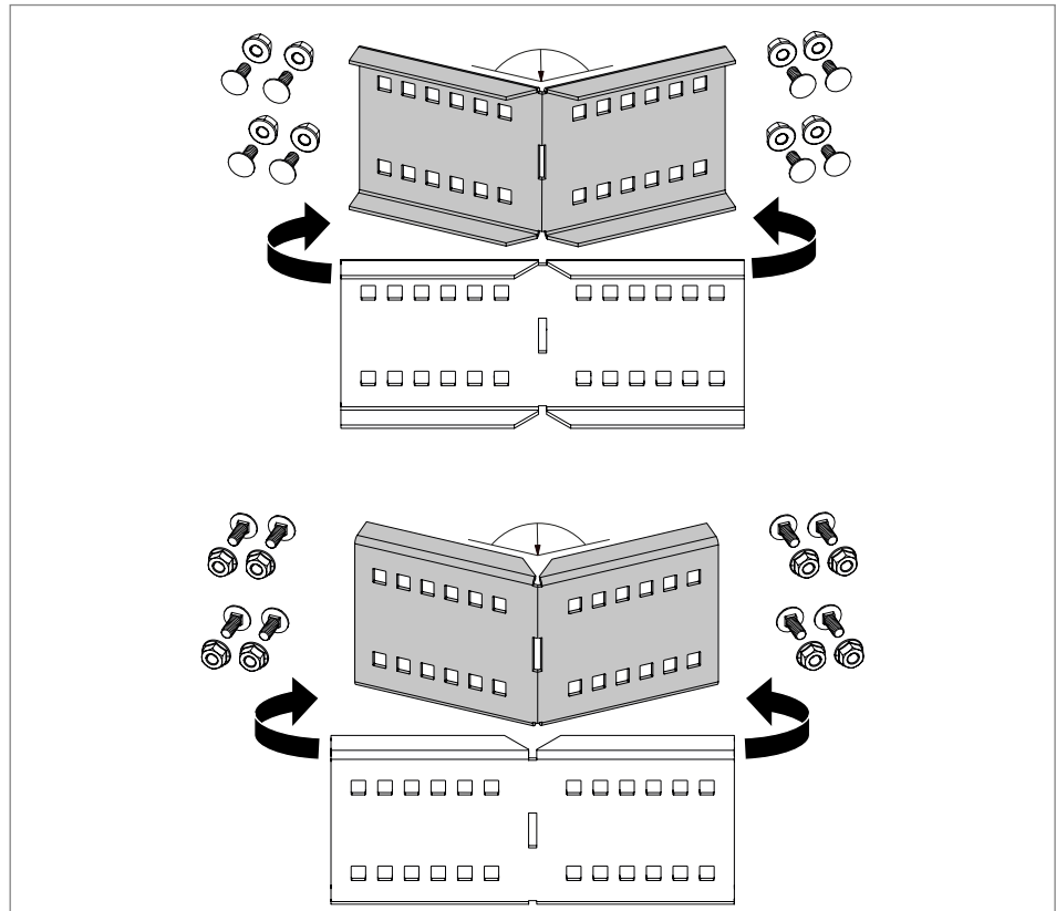
Fig. 17: Bending the WRWVK angle connector for inner and outer angles
