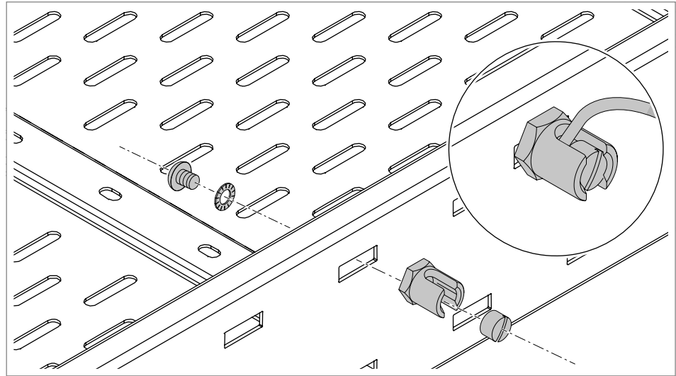
Fig. 50: Mounting the earthing terminal
