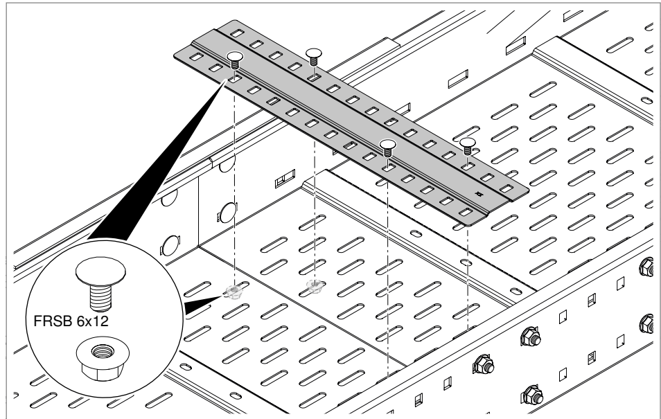
Fig. 12: Mounting the joint plate
