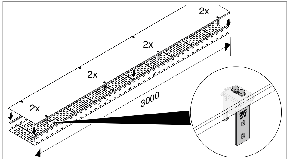
Fig. 48: Mounted spacer on DRL FAM cover
