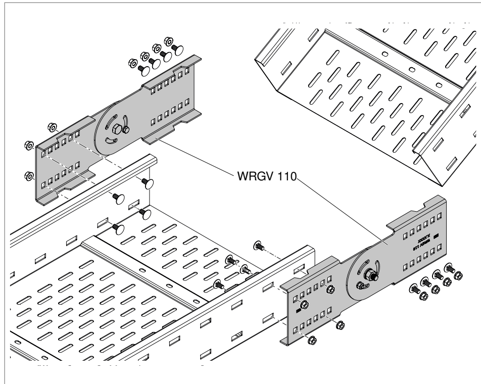
Fig. 22: Applying the adjustable connector
