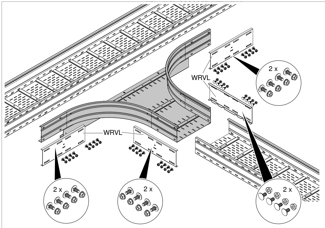
Fig. 35: Components for the mounting of an add-on tee
