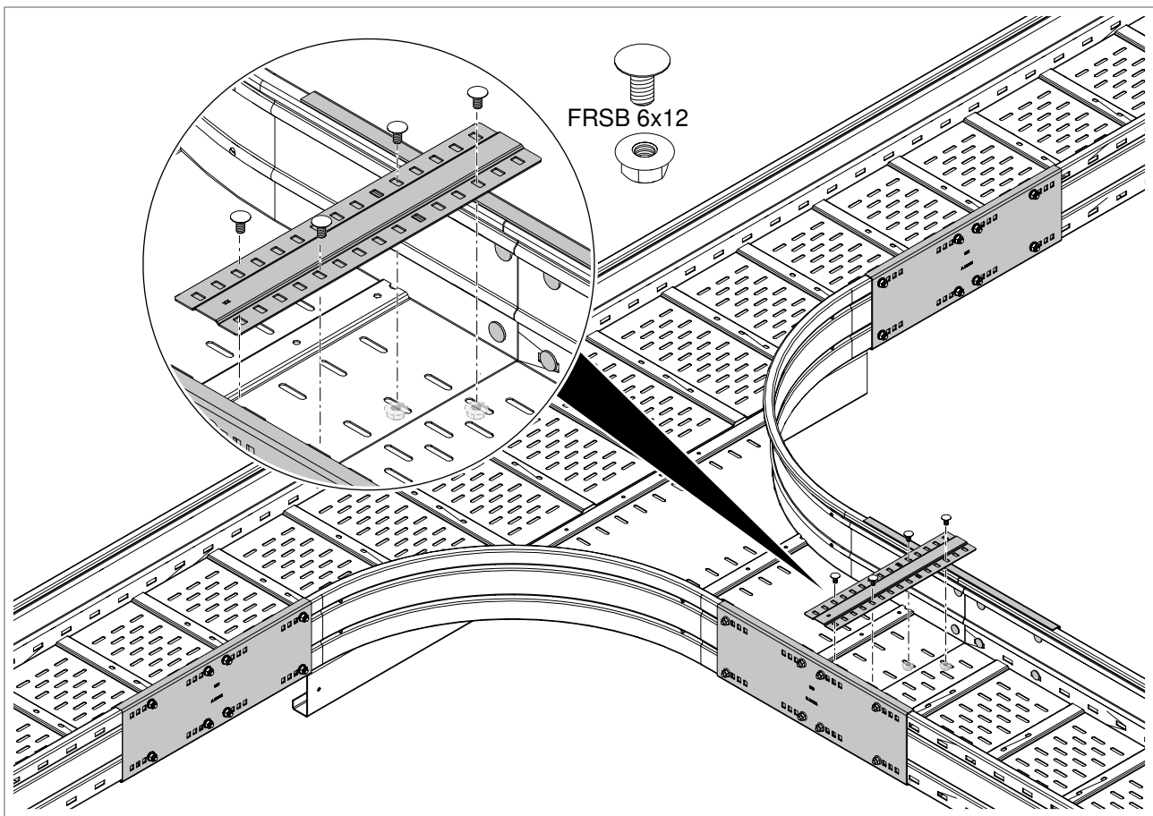
Fig. 38: Screwing on the joint plate
