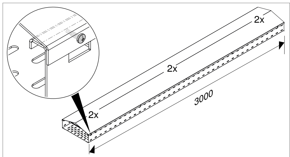
Fig. 44: Screwing on the cover at at least 6 points
