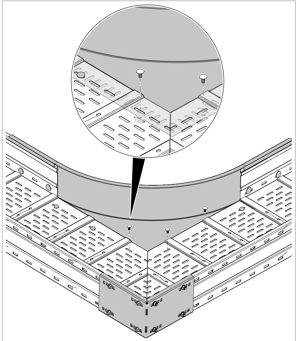
Fig. 42: Screwing on the joint plate
