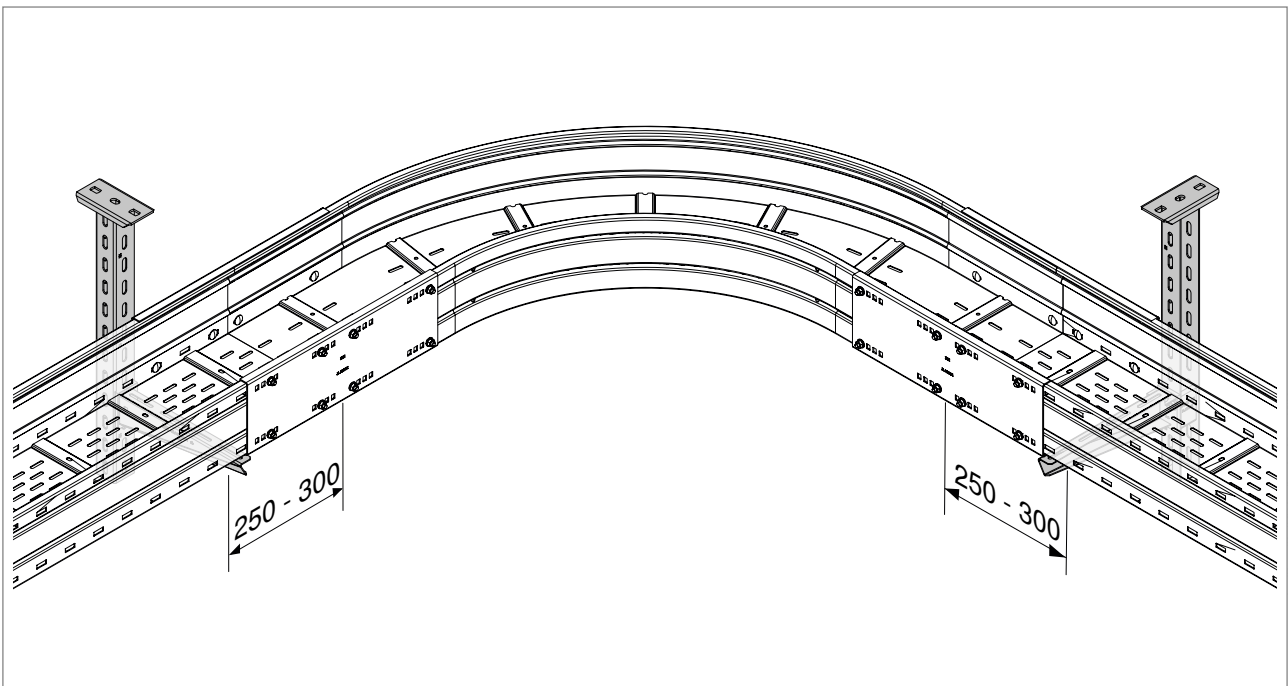
Fig. 30: Example of 90° bend fitting support with 300 mm width
