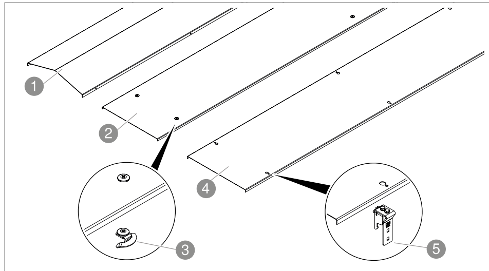
Fig. 7: Cover with fastening material
