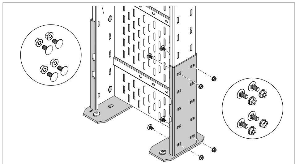
Fig. 29: Screwing the tray to the base plate
