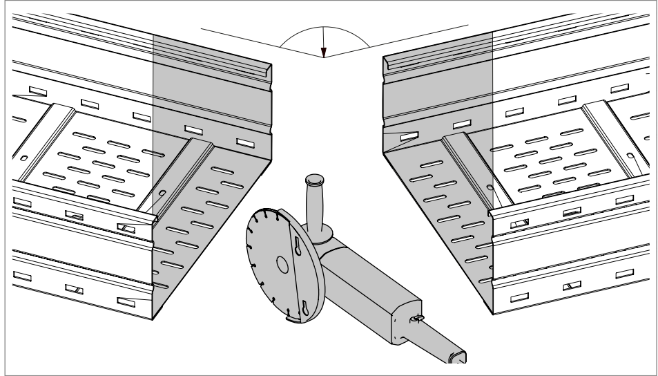
Fig. 16: Cutting the trays to create angles
