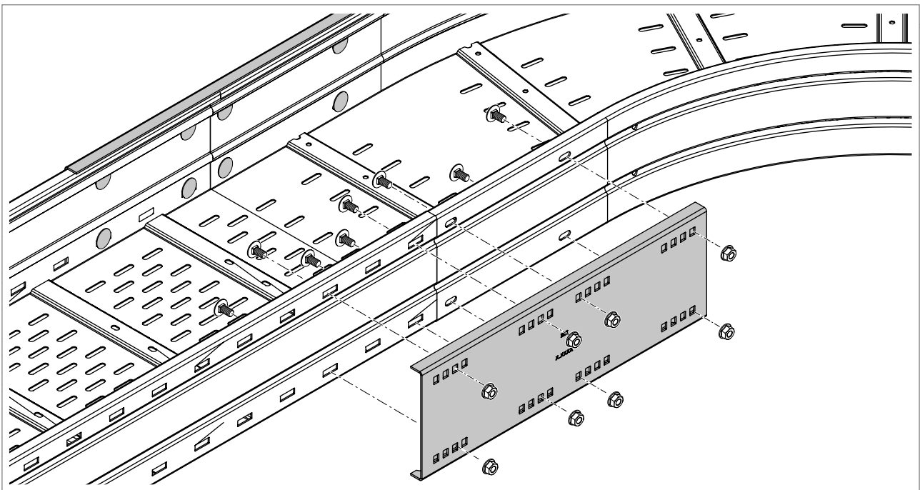
Fig. 33: Screwing on connectors
