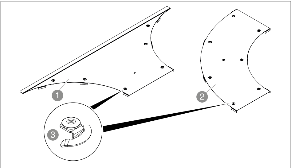
Fig. 8: Covers for fittings
