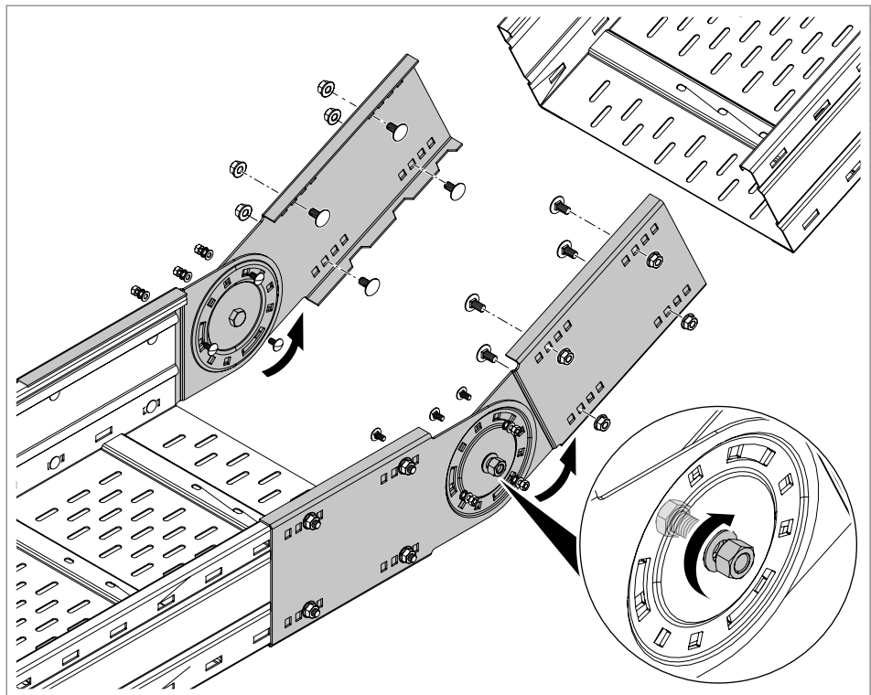
Fig. 26: Adjusting the angle
