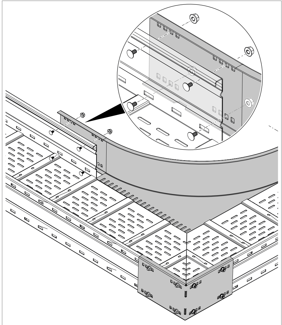
Fig. 41: Screwing on the corner extension piece and angle connector
